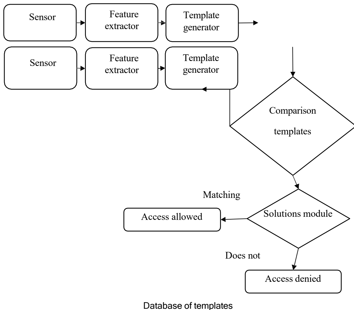
Fig. 2. Algorithm for bio-identification of user of a multi-user cloud system
